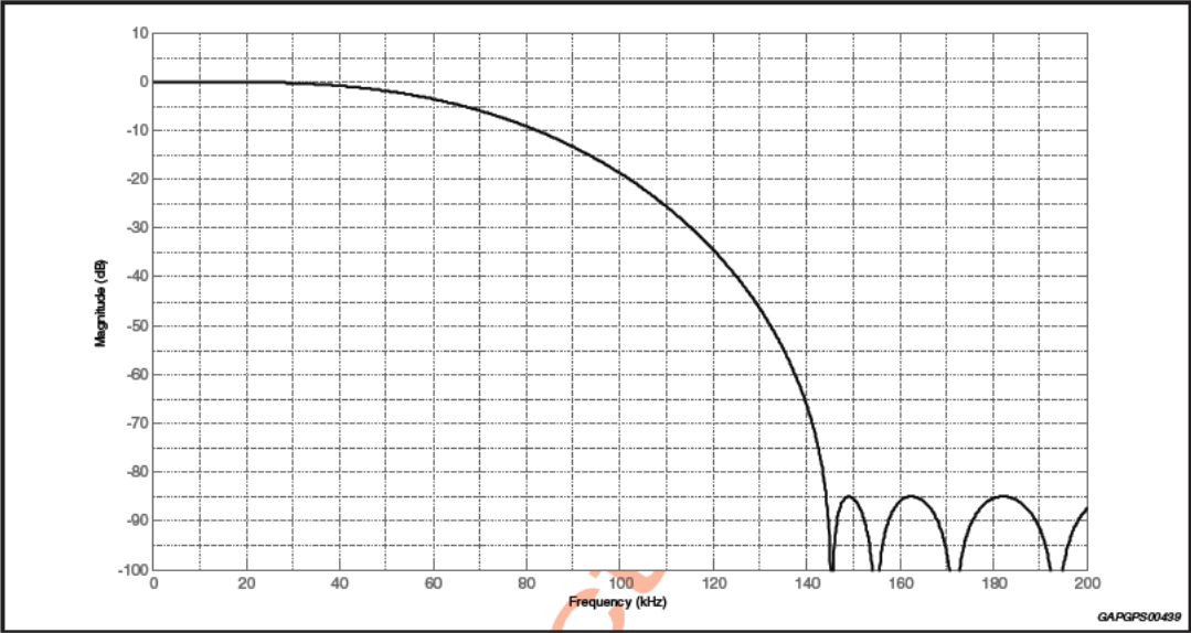
Figure 8. Cumulative digital-down-converter transfer function for AM
