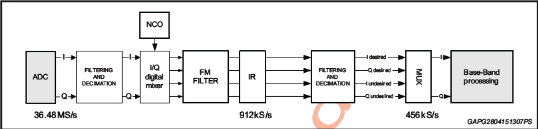
Figure 6. Digital-down-converter simplified block diagram
