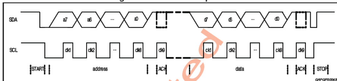
Figure 4. I 2 C "write" sequence
