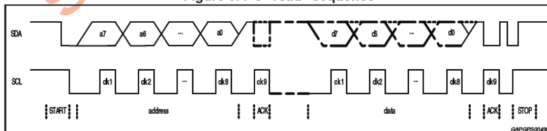
Figure 5. I 2 C "read" sequence
