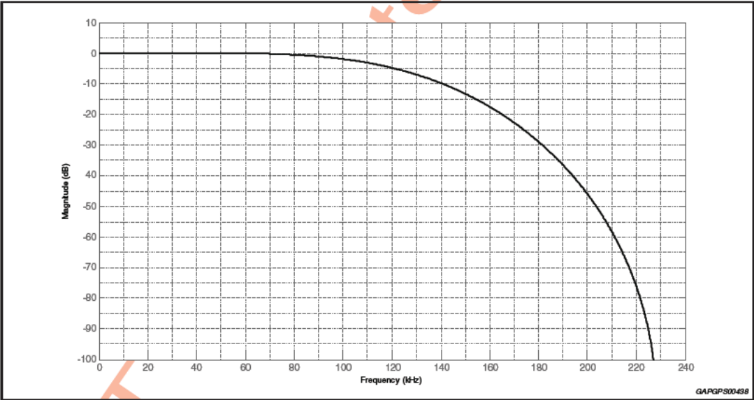
Figure 7. Cumulative digital-down-converter transfer function for FM
