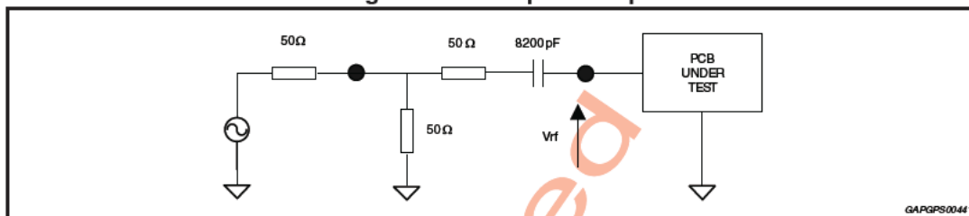
Figure 10. FM input set-up
